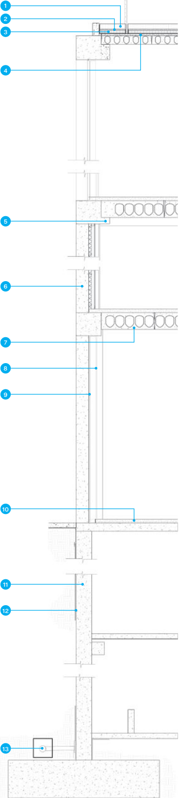
East Façade Section Detail
