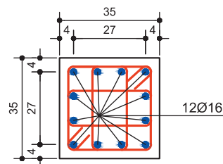
Section F-F
