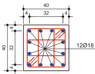
Section E-E
