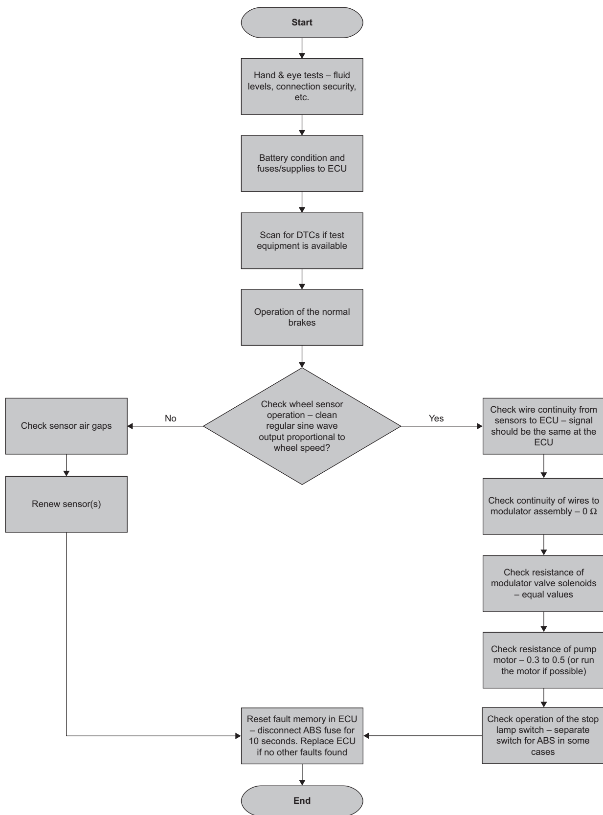
Figure 7.11 ABS diagnosis chart
