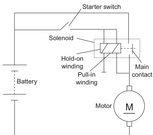
Figure 6.95 Starter circuit
