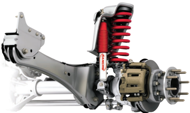
Figure 7.36 Suspension system (Source: Ford Media)
