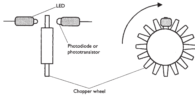
Figure 4.34 Optical sensor
