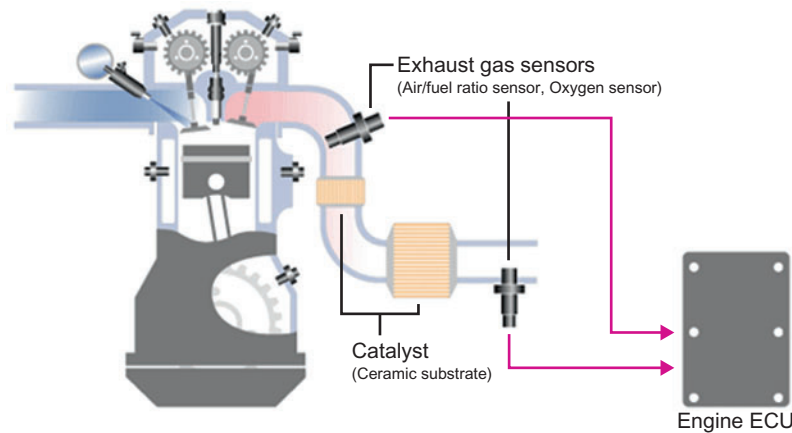
Figure 5.8 Exhaust gas oxygen sensors positioned pre- and post-catalyst (Source: http://www.globaldensoproducs.com )
