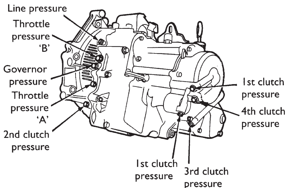
Figure 9.17 Transmission pressure testing points
