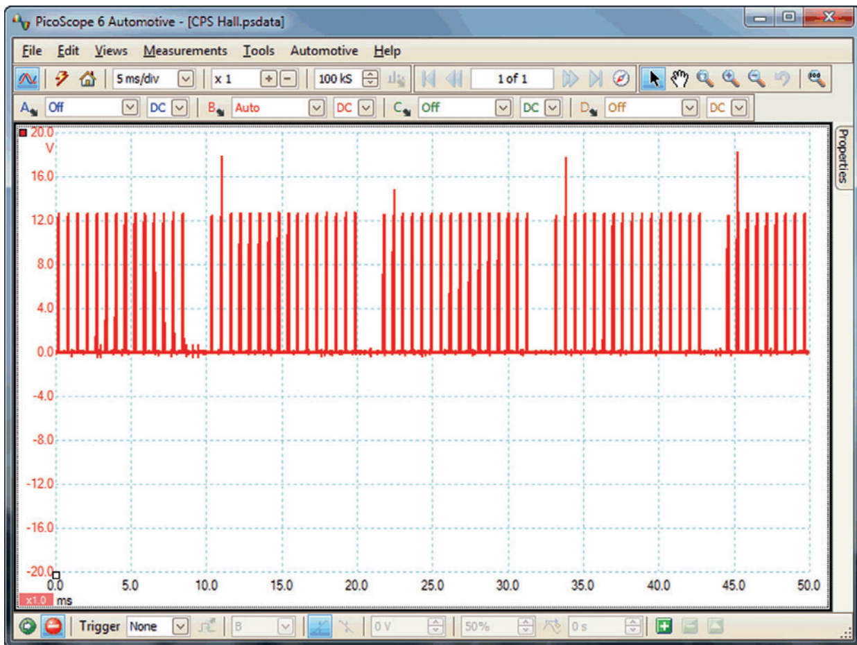
Figure 4.3 Hall effect crank sensor
