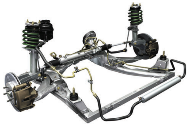
Figure 7.31 Front suspension struts (Source: Jaguar Media)
