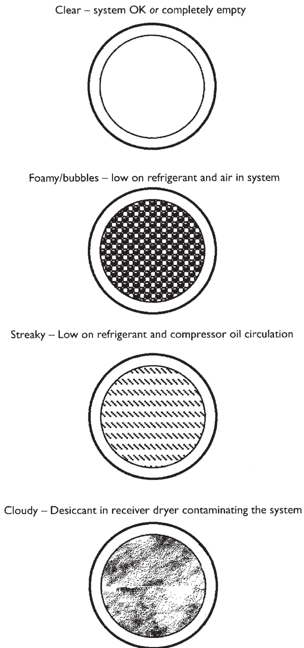
Figure 8.80 AC receiver sight glass
