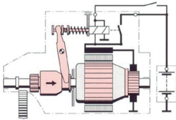
Figure 6.99 Starter circuit and engagement mechanism
