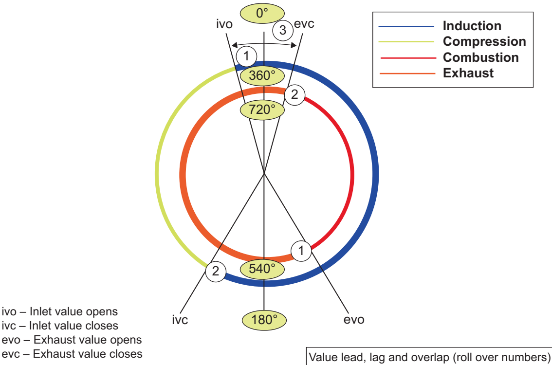
Figure 6.5 Valve timing diagrams (1 – lead; 2 – lag; 3 – overlap)
