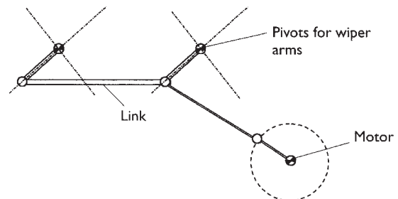
Figure 8.33 Wiper linkage
