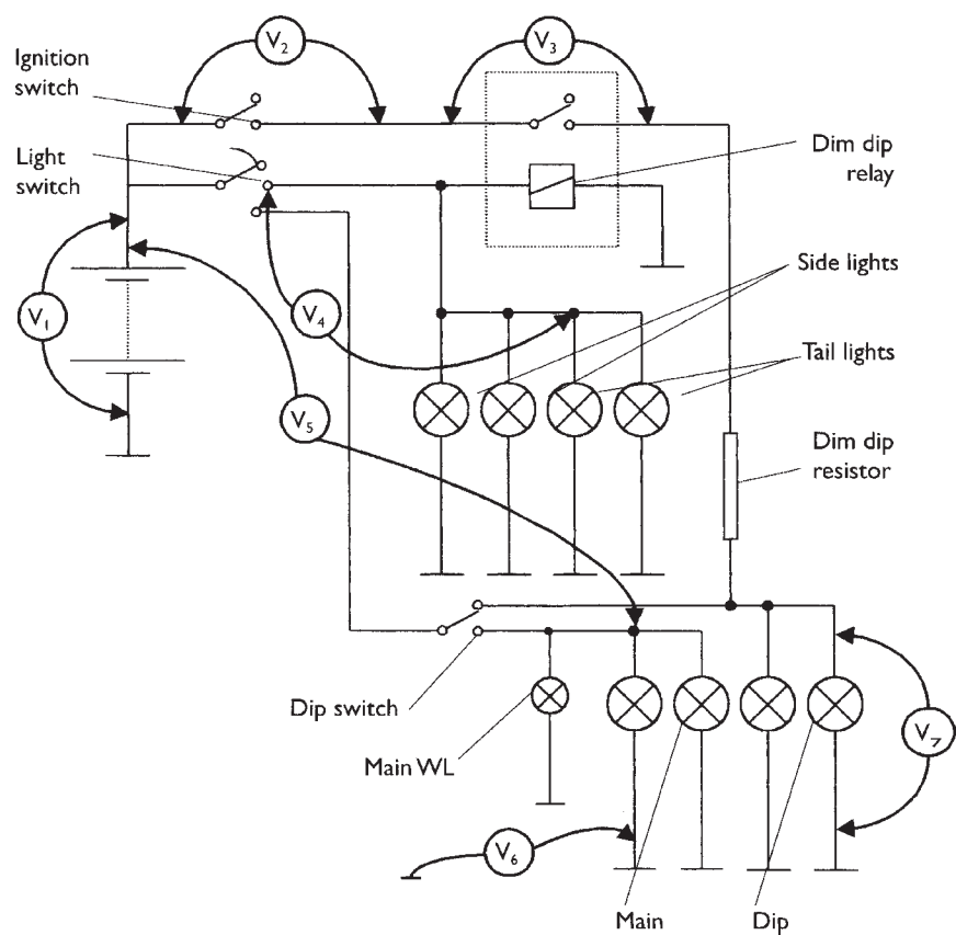
Figure 8.29 Lighting circuit under test
