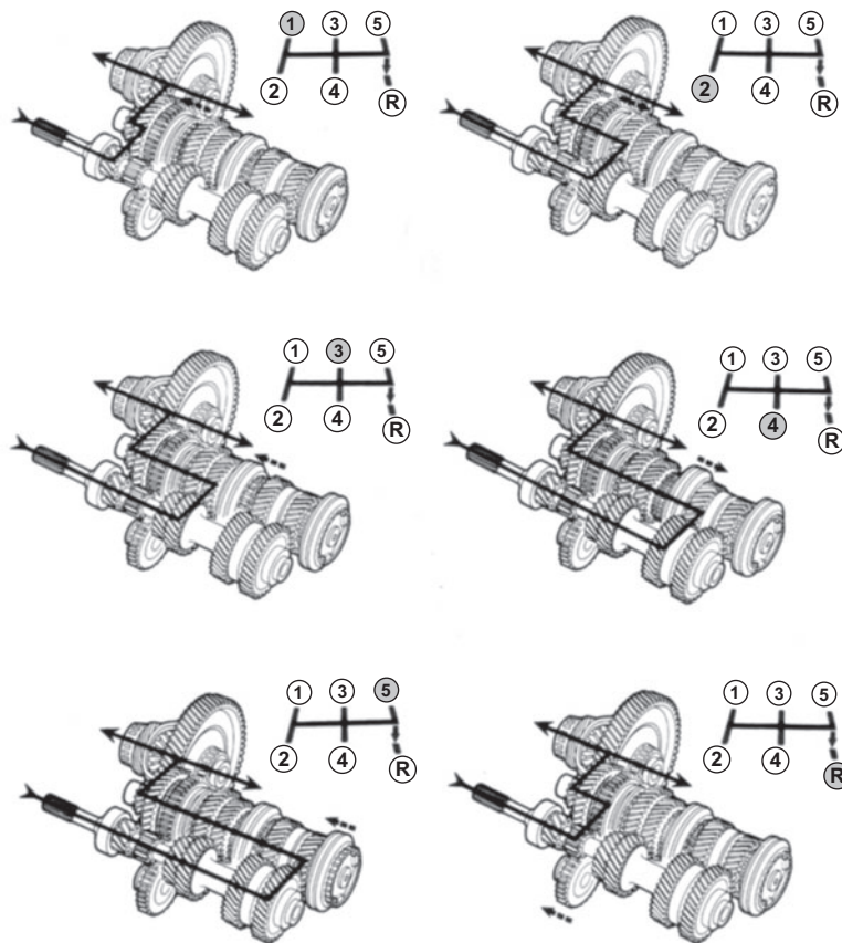
Figure 9.4 Five-speed manual gearbox and power flows
