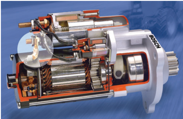
Figure 6.103 The link from the solenoid contacts and the motor is highlighted in this image
