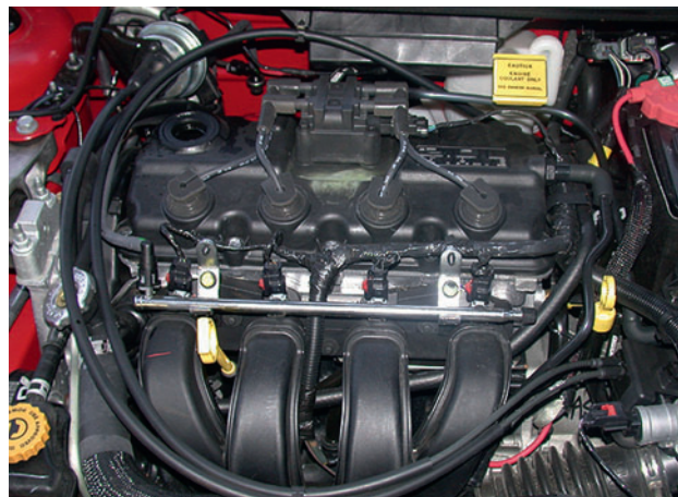
Figure 6.25 DIS coil on a four-cylinder engine
