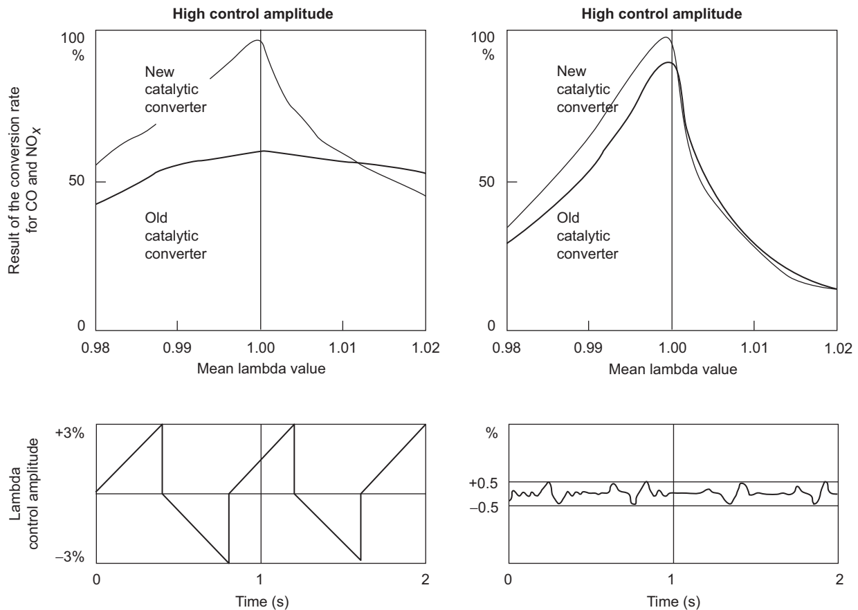
Figure 6.56 Effect of lambda control on catalytic converters
