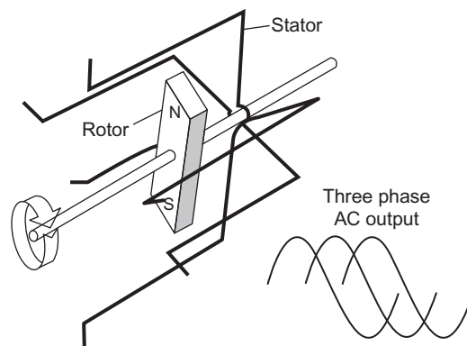
Figure 6.105 Alternator principle
