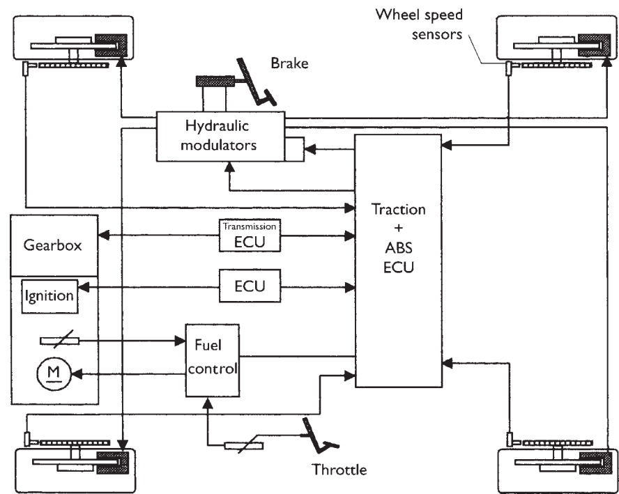
Figure 7.13 Integrated traction control system
