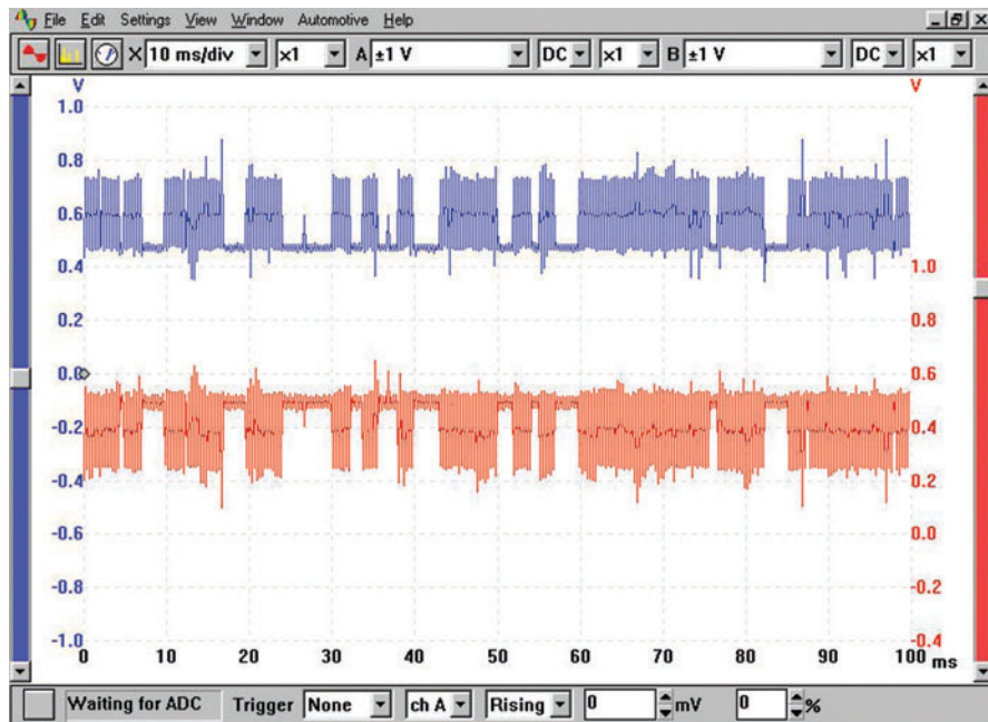
Figure 8.17 CAN signals
