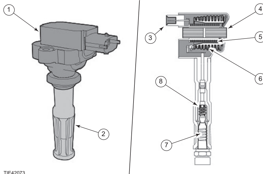
Figure 6.26 Direct ignition coil features: 1 – direct ignition coil; 2 – spark plug connector; 3 – low-voltage connection; outer: 4 – laminated iron core; 5 – primary winding; 6 – secondary winding; 7 – spark plug; 8 – high-voltage connection; inner: via spring contact (Source: Ford Motor Company)
