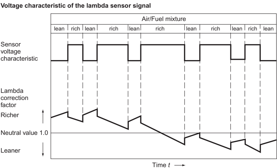
Figure 5.12 Rich AFR lambda sensor signal fuelling error (Source: Bosch)
