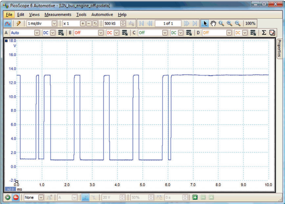
Figure 4.71 LIN waveform
