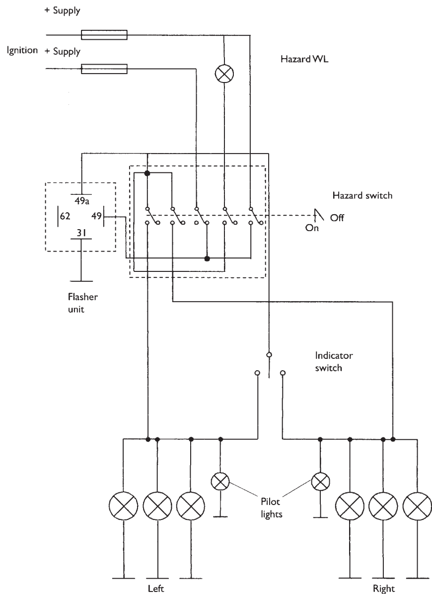
Figure 8.39 Indicator and hazard circuit
