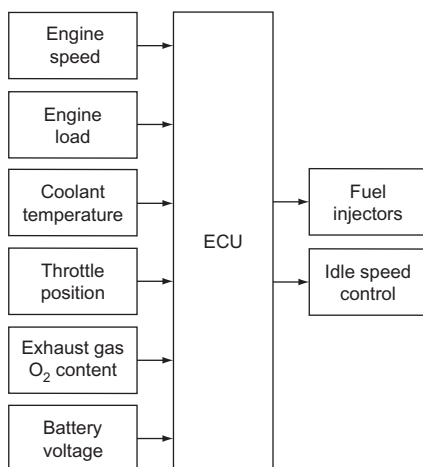
Figure 6.44 Fuel injection simplified block diagram
