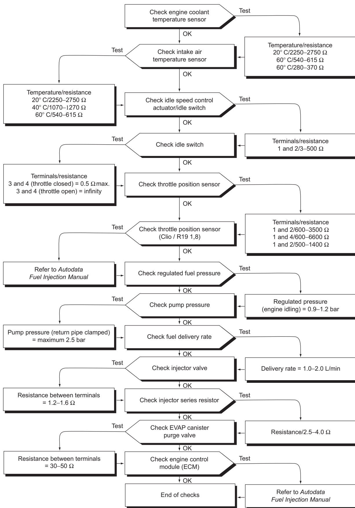
Figure 6.75 Faultfinding chart
