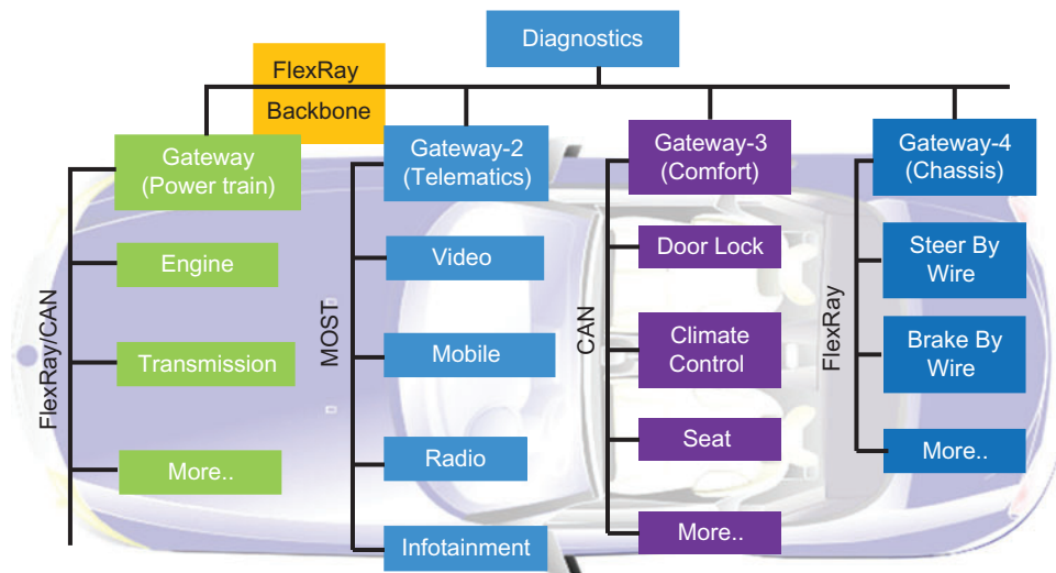
Figure 8.15 FlexRay backbone
