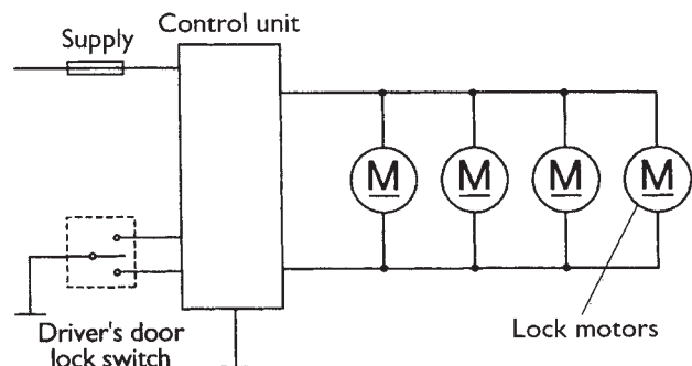
Figure 8.57 Door lock circuit
