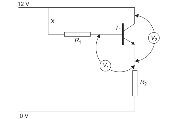
Figure 8.4 Transistor testing: Use resistors R_1 = R_2 of approximately 1 k \Omega , when connected as shown, V_1 should read 0.6–0.7V and V_2 approximately 1V. Disconnect wire X, V_1 should now read 0V and V_2 12V
