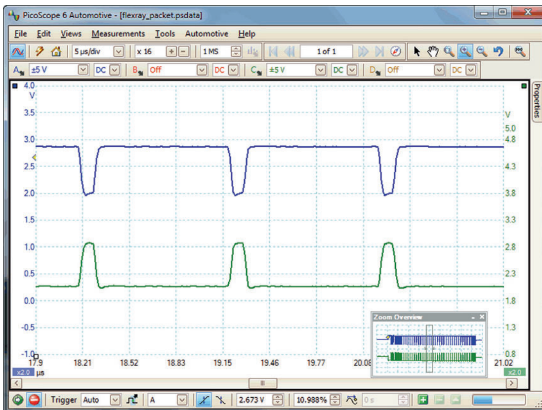
Figure 4.73 A closer view of a FlexRay signal
