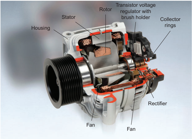
Figure 6.104 Alternator components
