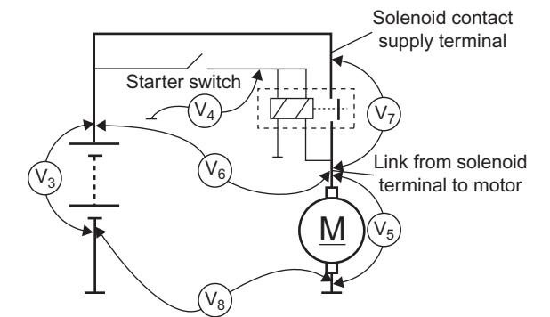
Figure 6.102 Starter circuit testing
