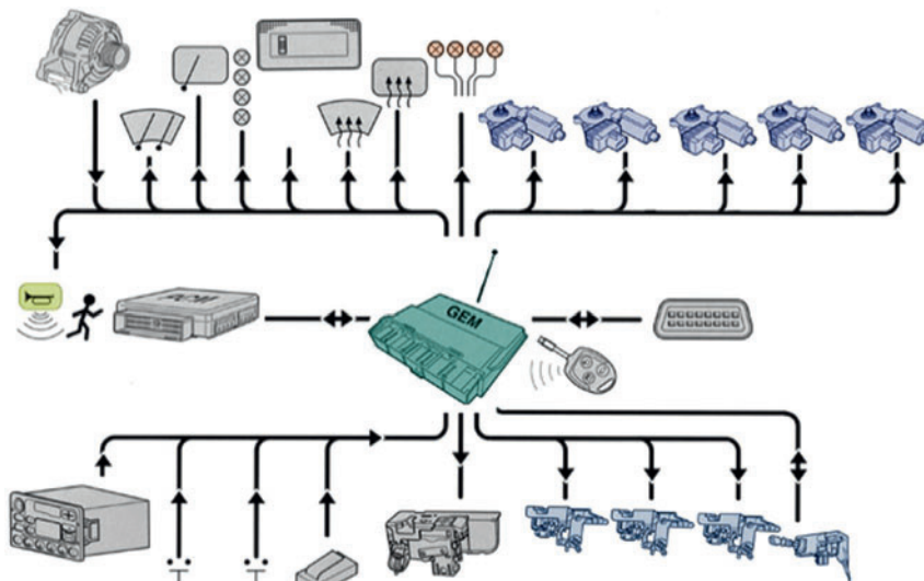
Figure 8.37 GEM and components (Source: Ford Motor Company)
