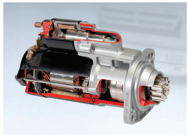
Figure 6.97 Intermediate transmission starter (Source: Bosch Media)
