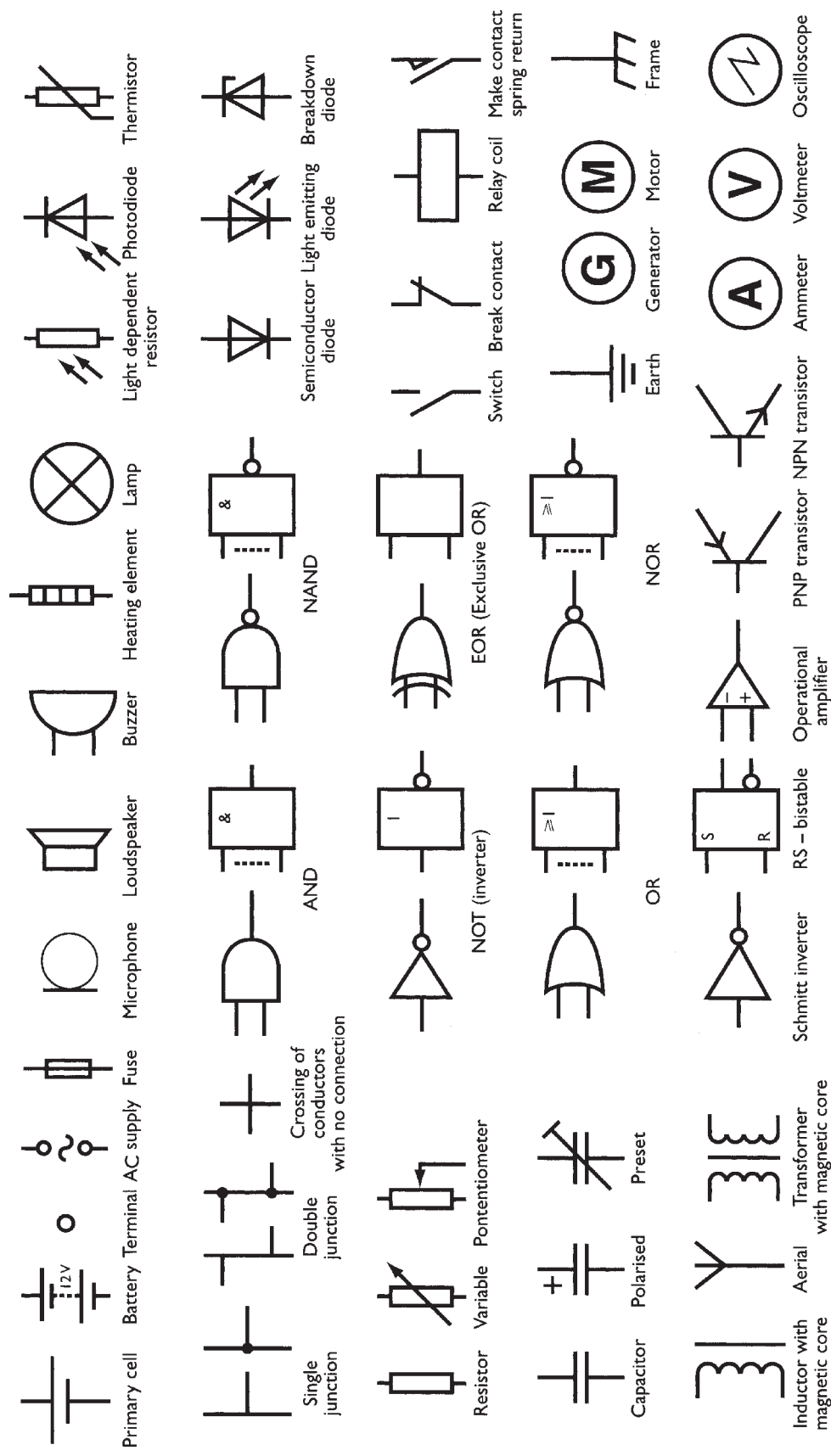
Figure 8.1 Circuit symbols
