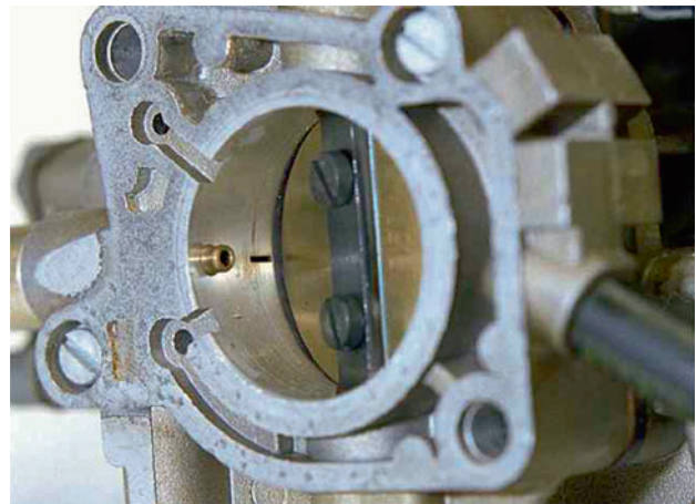
Figure 6.9 Throttle butterfly
