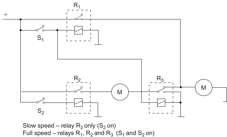
Figure 8.43 Two-speed, twin cooling fan circuit
