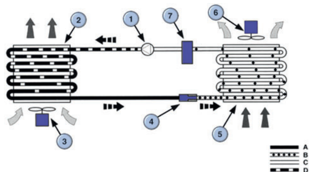
Figure 8.74 AC system layout: 1 – compressor; 2 – condenser; 3 – auxiliary fan (depending on model); 4 – fixed orifice tube; 5 – evaporator; 6 – heater/air conditioning blower; 7 – suction accumulator/drier; A – high-pressure warm liquid; B – low-pressure cool liquid; C – low-pressure, gaseous and cool; D – high-pressure, gaseous and hot (Source: Ford Motor Company)
