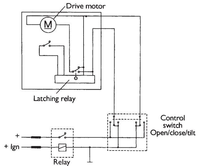
Figure 8.56 Sunroof circuit example
