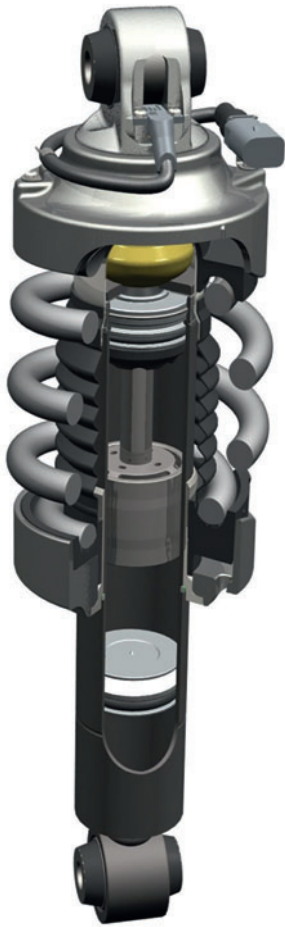
Figure 7.40 Suspension strut and actuator connection (Source: Delphi Media)
