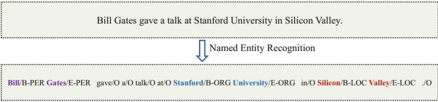
Fig. 5.1 An example of named entity recognition, in which we use “B”, “M”, “E” and “O” to denote “Begin”, “Middle”, “End” and “Out” of a named entity
