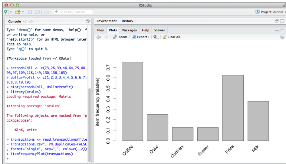
Figure 12-10: Transaction frequencies
