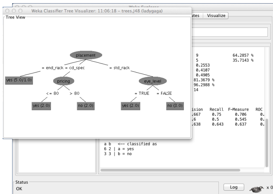
Figure 3-7: J48 visualization
