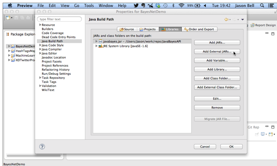
Figure 4-7: Project properties
