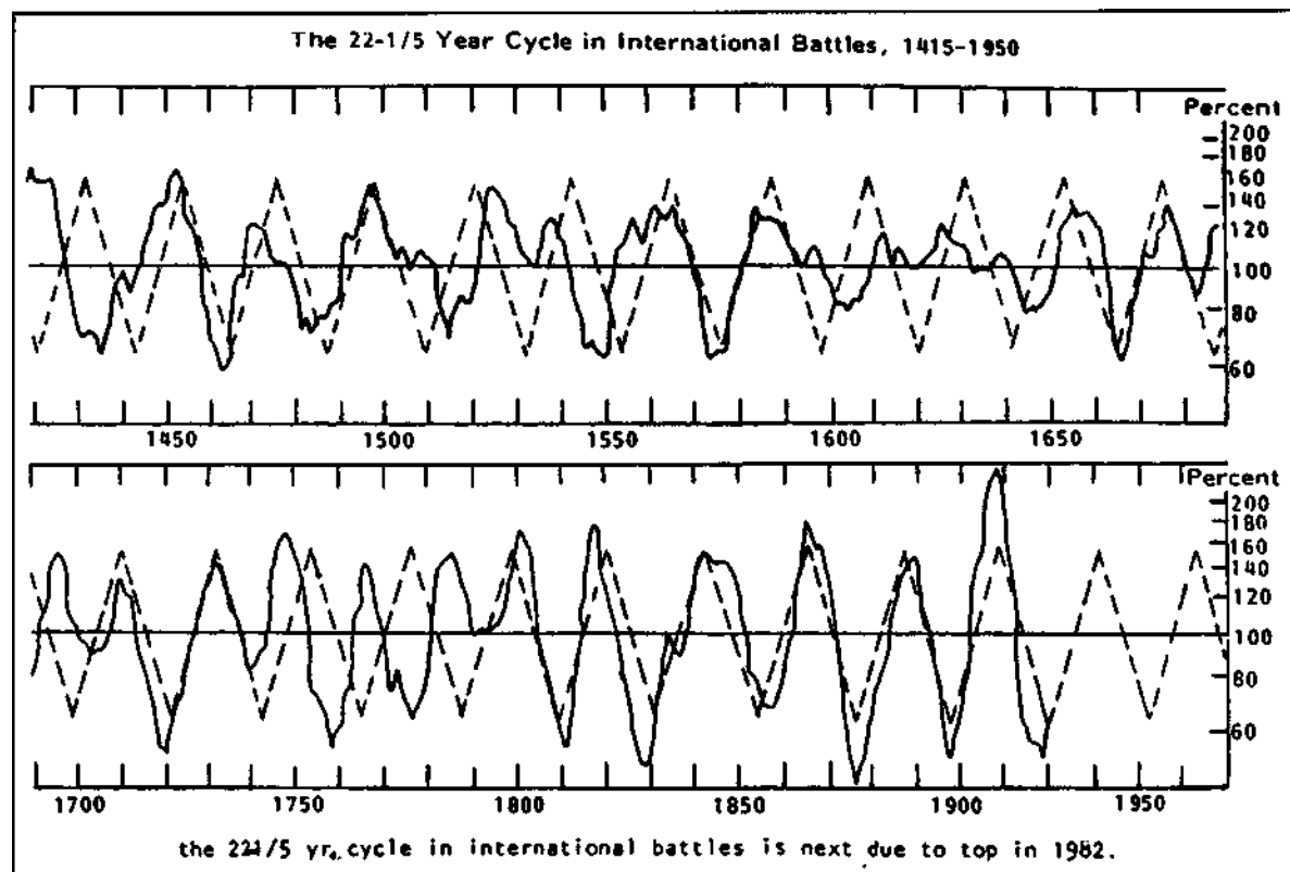
Figure 14.2 The 22.2 year cycle in international battles was due to top in 1982. In the chart the dotted line is the "ideal" cycle, and the solid line is the actual detrended data. (Courtesy of the Foundation for the Study of Cycles, Wayne, PA.)
